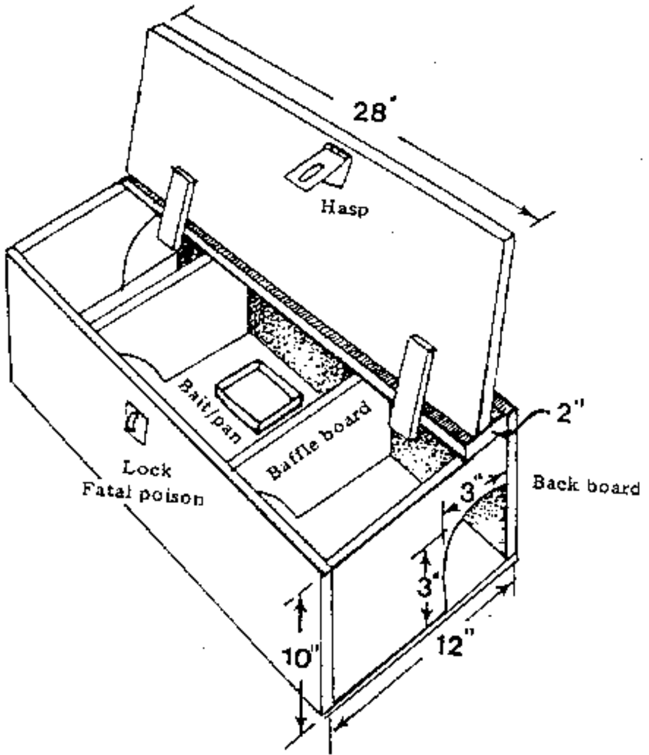
Figure 7. Plans for a do-it-yourself wooden, tamper-resistant bait station.
